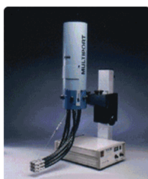
SPF Testing 601-300W Multiport UV Solar Simulator Installed at SUNJIN in 2009
